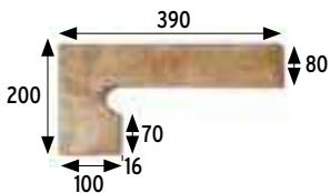
Zanquín izda./dcha. String left/right side 390x80/200x100x16 mm
