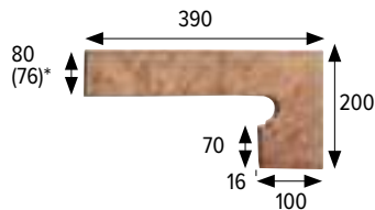
Zanquín dcha. String right side 390x80/200x100x16 mm
