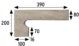
Zanquín izda. String leftside 390x80/200x100x16 mm
