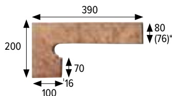
Zanquín izda. String leftside 390x80/200x100x16 mm
