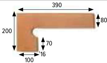
Zanquín izda. String leftside 390x80/200x100x16 mm
